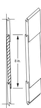
8 in. Sure Lock 1/2 in. Lap Siding 9.33 sq. ft. coverage/piece
